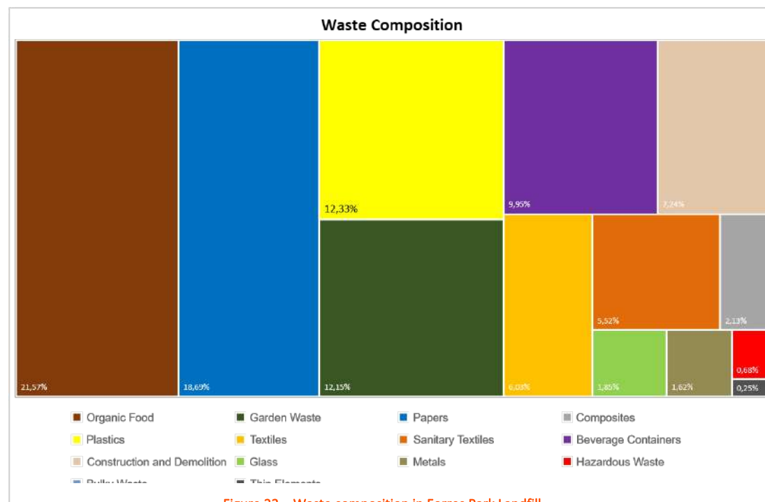
Figure 23 – Waste composition in Forres Park Landfill
