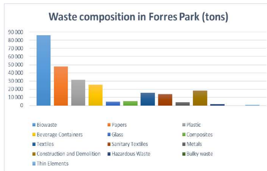
Figure 22– Waste composition in Forres Park Landfill (tons)
