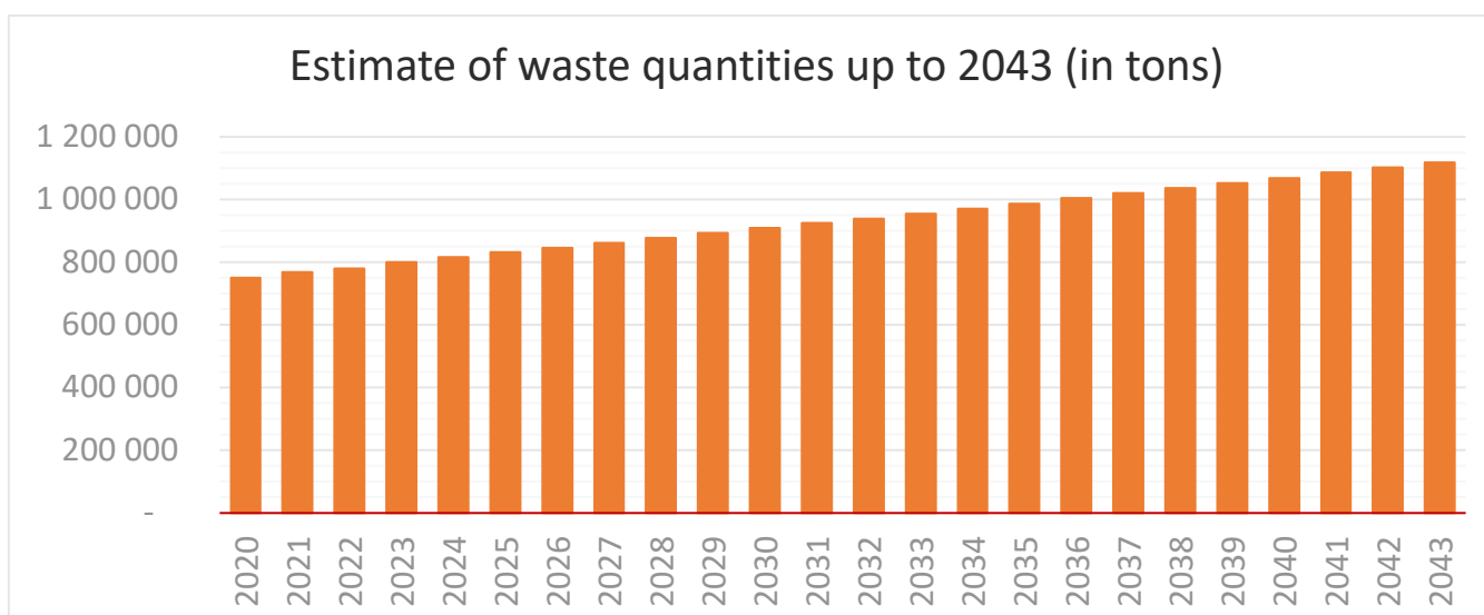
Figure 39– Estimation of the waste production until 2043
